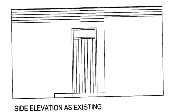
SIDE ELEVATION AS EXISTING
